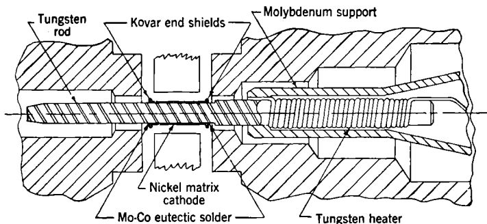
FIG. 12-33.—Oxide matrix cathode of the 3J21. (2X.)
